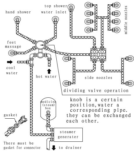
BACK SIDE WATER CONNECTION WAY
