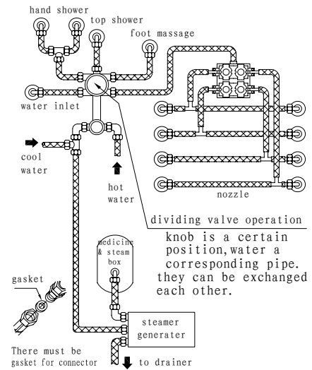
BACK SIDE WATER CONNECTION WAY
