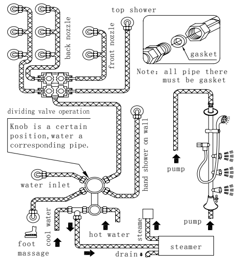
BACK SIDE WATER CONNECTION WAY
